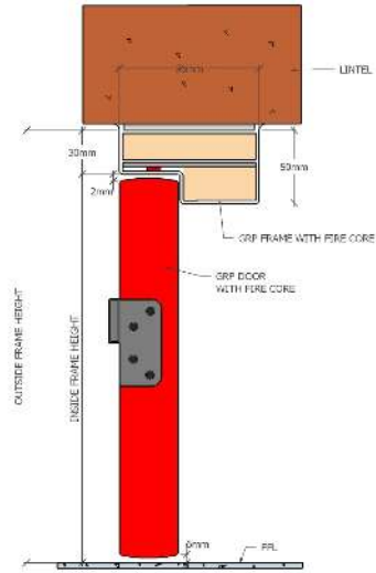
Side section, fixed to GRP frame detail
