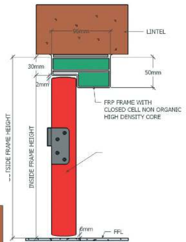
Side section, fixed to FRP frame detail
