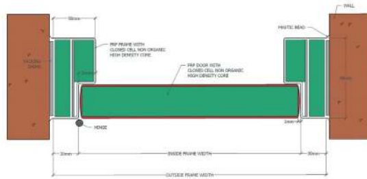
Right hand hung blade, fixed to FRP frame
