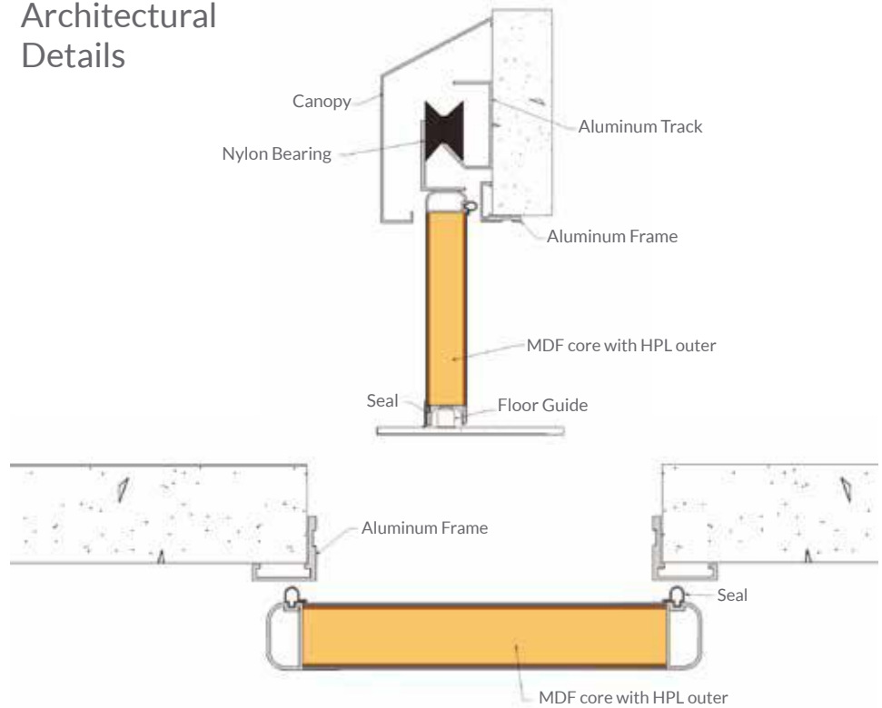
Hermetic sliding door, fixed to aluminum frame
