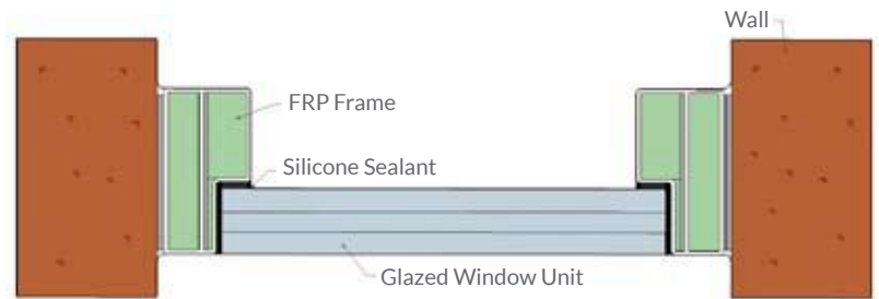
FRP Framed Window
